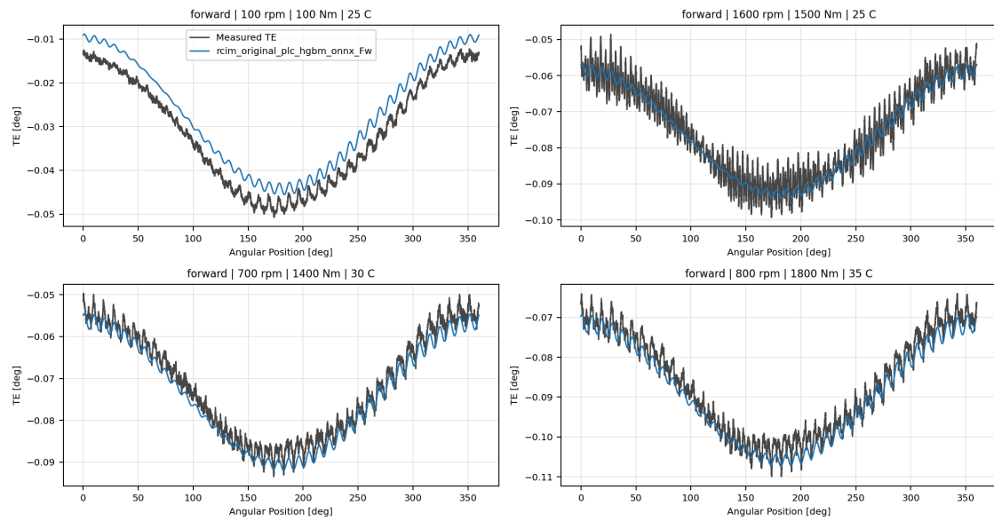
rcim_original_plc_hgbm_onnx_Fw curve-verification collage
