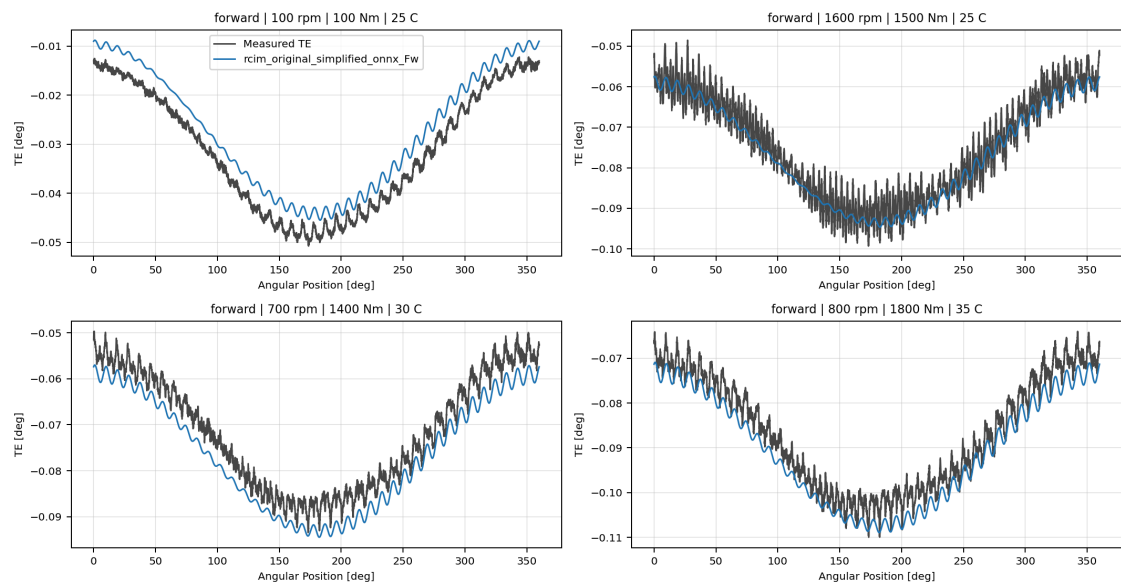
rcim_original_simplified_onnx_Fw curve-verification collage
