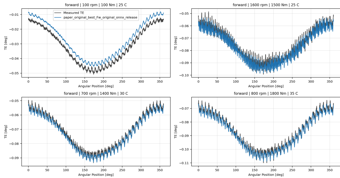
paper_original_best_Fw_original_onnx_release curve-verification collage
